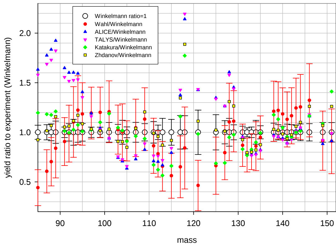
Benchmark A: ^{242}\text{Pu} at 15.1 MeV, post neutron emission yield ratio to experiment (Winkelmann)
