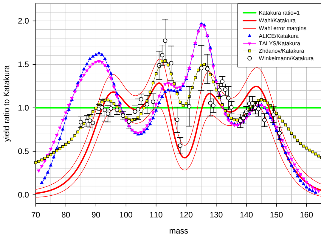
Benchmark A: ^{242}\text{Pu} at 15.1 MeV post neutron emission fission yield ratios to Katakura
